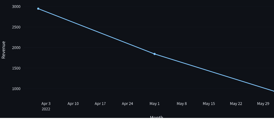
Monthly Revenue
