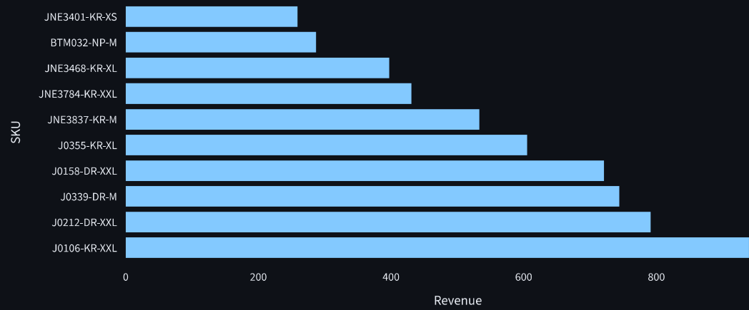
Top 10 Products
